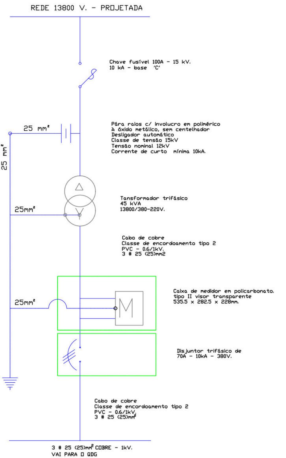
DIAGRAMA UNIFILAR
