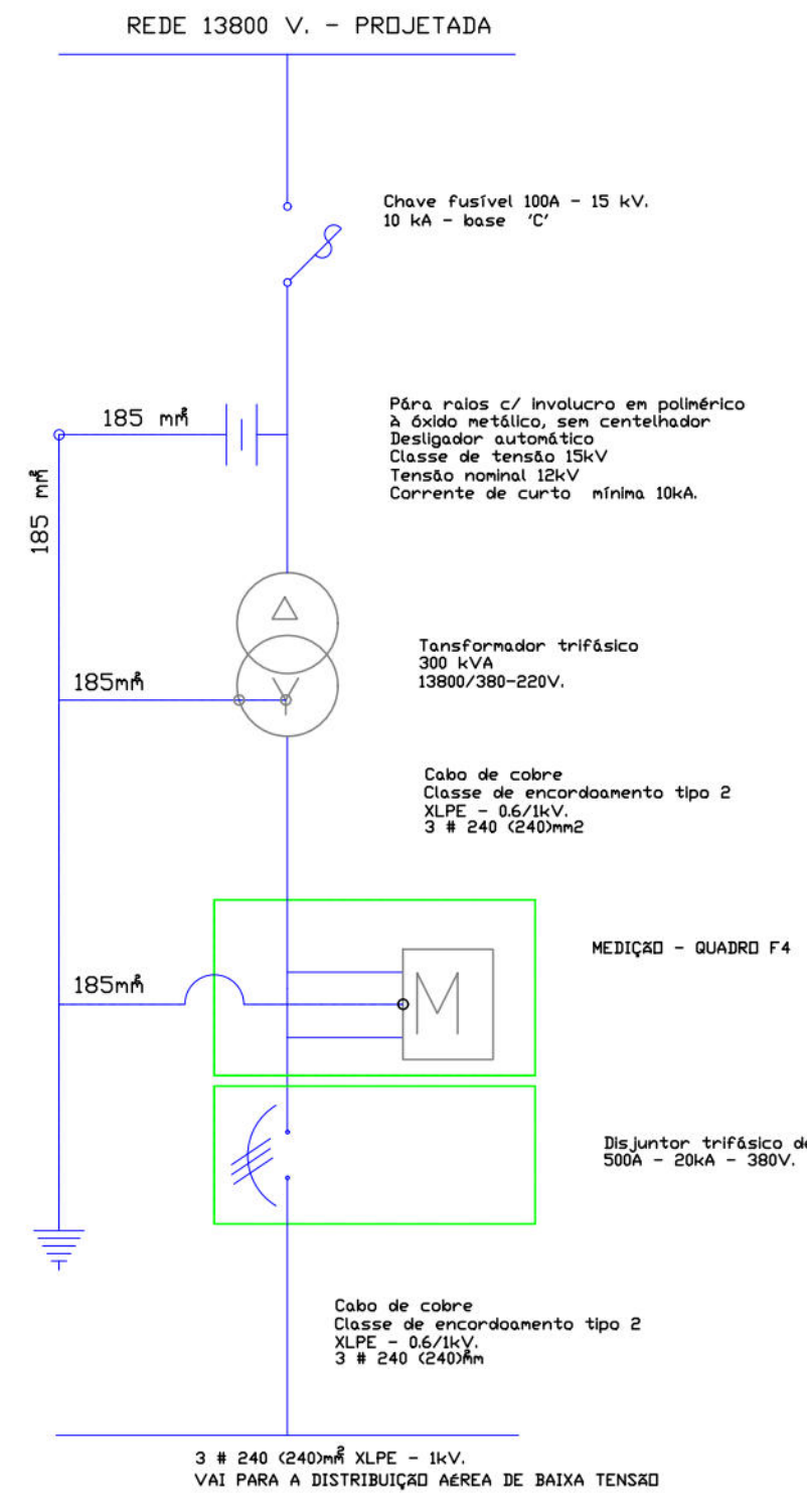
DIAGRAMA UNIFILAR
