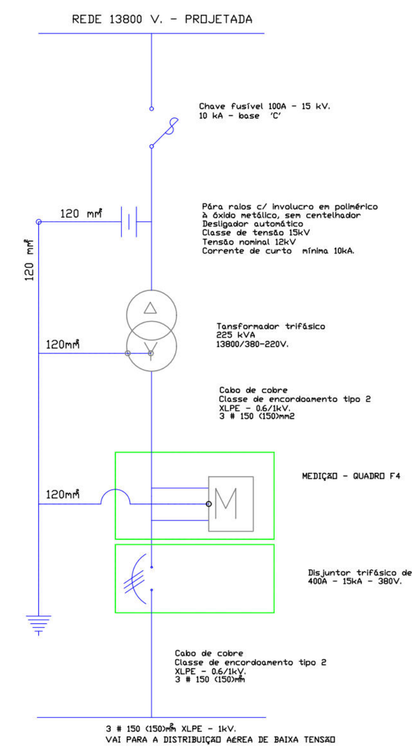
DIAGRAMA UNIFILAR
